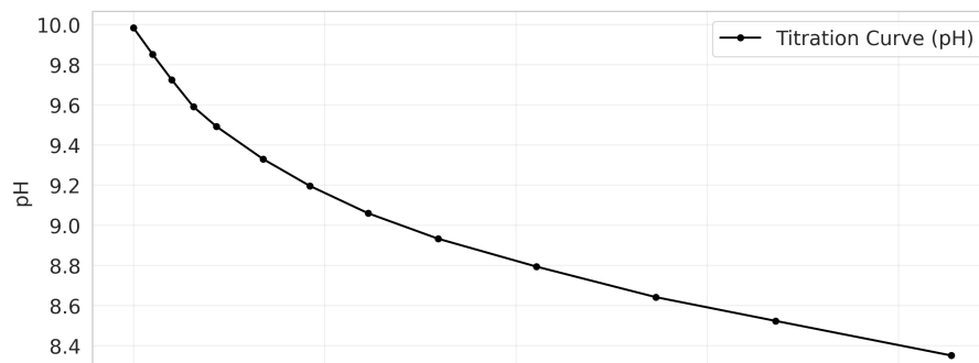
Opt Schwartz EQP = 6.698 mL, k = 0.000
