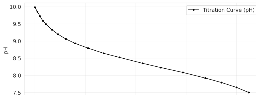
Opt Schwartz EQP = 5.108 mL, k = 0.000
