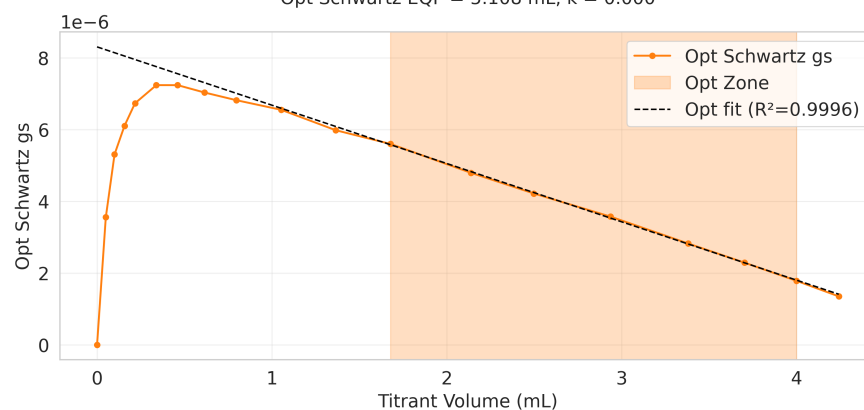
Opt Schwartz EQP = 5.108 mL, k = 0.000
