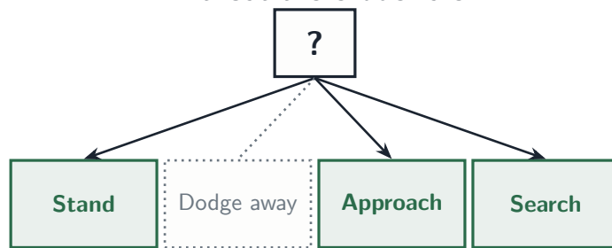
Without the evade rule
