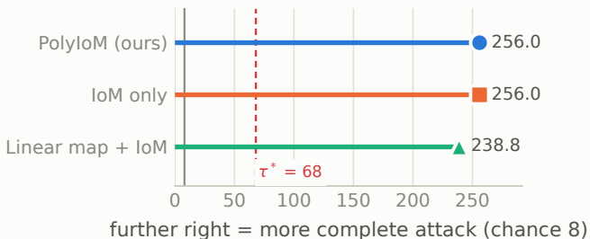
face — matching positions reached (of 256)
