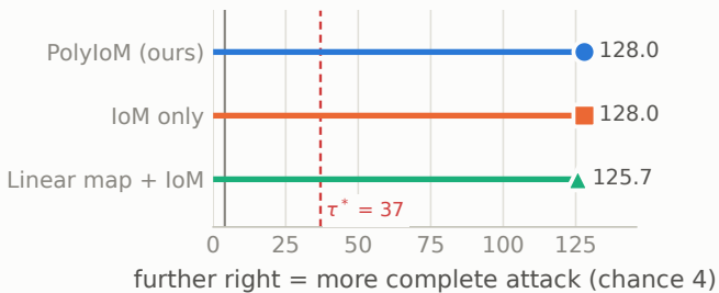
voice — matching positions reached (of 128)
