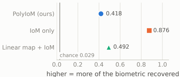
face — cosine to the true embedding
