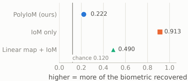
voice — cosine to the true embedding
