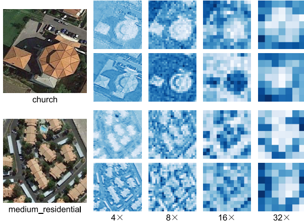
Fig. 7. Visualization of feature maps of 4 \times , 8 \times , 16 \times , and 32 \times DSLs with Swin V2-Tiny init and +RFD models. Church and medium_residential are input images. The first and third rows are excerpts of downsampled feature maps at different scales of the Swin V2-Tiny network. The second and fourth rows are excerpts of downsampled features at different scales for the Swin V2-Tiny + RFD network.
