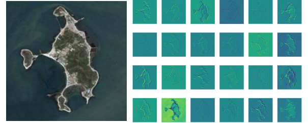
Fig. 5. Visualization of feature maps after feature reinforcement layer in Swin V2-Tiny + RFD.
