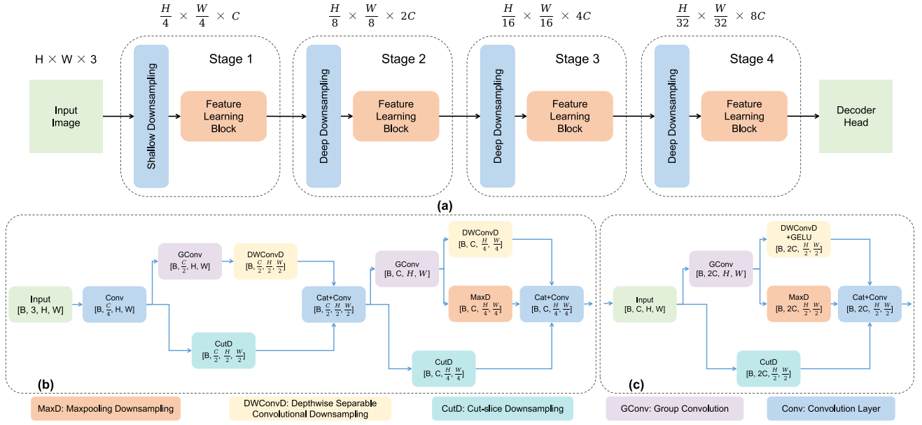
Fig. 3. Overall architecture of the proposed RFD. (a) General structure after replacement with SRFD and DRFD modules. (b) and (c) Details of SRFD and DRFD modules, respectively.
