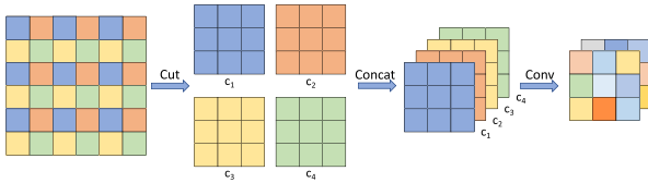
Fig. 4. Cut-slice downsampling. Cut denotes slicing adjacent pixel points into c_1 , c_2 , c_3 , and c_4 . Concat denotes concatenating feature maps \{c_1, c_2, c_3 , and c_4\} . Conv denotes a 1 \times 1 convolution with stride 1 and the number of channels reduces from 4C to 2C .
