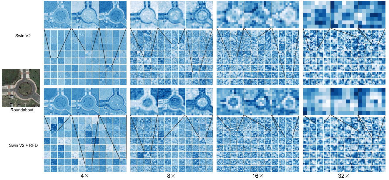
Fig. 6. Visualization of feature maps of 4\times , 8\times , 16\times , and 32\times DSLs with different models. Roundabout is the input image. Swin V2 and Swin V2 + RFD denote initial and +RFD models of Swin V2-Tiny, respectively. The test image is randomly selected from the validation set of NWPU-RESISC45, and only the first 96 channels are listed for each layer visualization.
