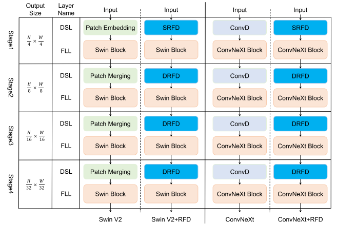
Fig. 2. Illustration of the proposed RFD module replacing DSLs in swin transformer V2 and ConvNeXt models. “+RFD” represents that the DSLs of the model are replaced by the RFD module. The SRFD module and the DRFD module are used to replace the stage 1 DSL and stage 2–4 DSLs of the original backbone networks, respectively. ConvD denotes convolutional downsampling. DSL denotes the downsampling layer. FLL denotes the feature learning layer.
