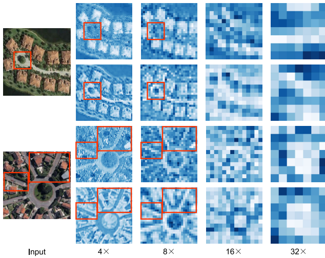
Fig. 1. Visualization of feature map of Swin V2 tiny init and +RFD models. The input images include dense residential and roundabouts. The first and third rows are excerpts of downsampled feature maps at different scales of Swin V2 tiny init. The second and fourth rows are excerpts of downsampled features at different scales for Swin V2 tiny + RFD. 4 \times , 8 \times , 16 \times , and 32 \times represent multiples of downsampling, respectively. The test images are randomly selected from the validation set of NWPU-RESISC45. For display purposes, we selected features that are friendly to human vision.
