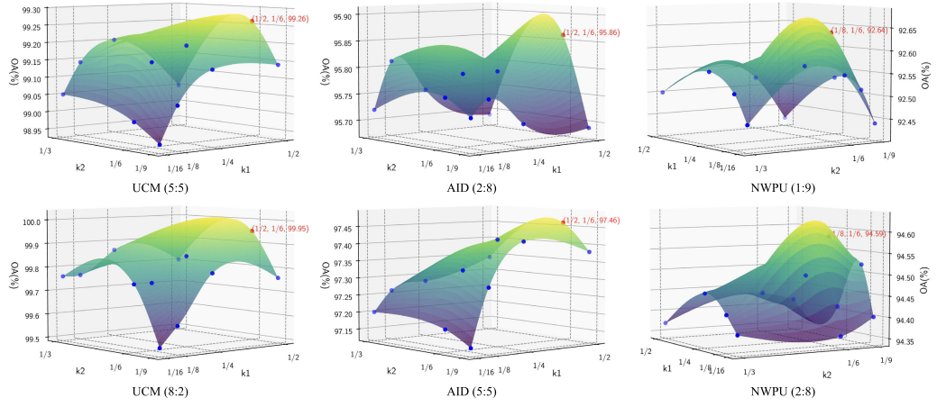
Fig. 11. OA values of MSCN with different k_1 and k_2 in MSC counted on the UCM, AID, and NWPU datasets. We fit the experimental results into a 3-D graph, where the data points corresponding to different values of k_1 and k_2 are indicated by blue dots. The maximum value is highlighted with a red dot, and its coordinates are annotated.
