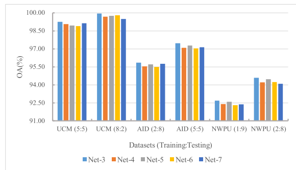
Fig. 18. OA values of Net-3 to Net-7 on the UCM, AID, and NWPU datasets.
