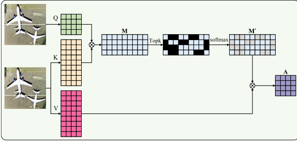
Fig. 5. Illustration of TopK sparse operation. Black color represents the value of -\infty , while gray indicates the value of 0.
