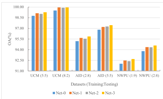
Fig. 17. OA values of Net-0 to Net-3 on the UCM, AID, and NWPU datasets.
