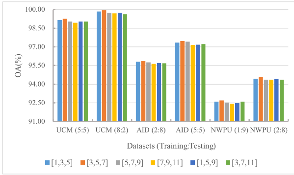
Fig. 10. OA values of different MSCNs with various pooling window sizes counted on the UCM, AID, and NWPU datasets.
