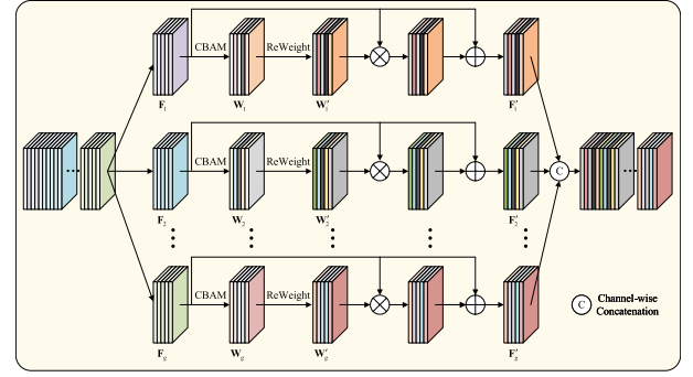
Fig. 6. Flowchart of the proposed GCE, which applies CBAM in a grouped manner to identify local salient information. Additionally, it readjusts the CBAM weights to highlight critical information further.
