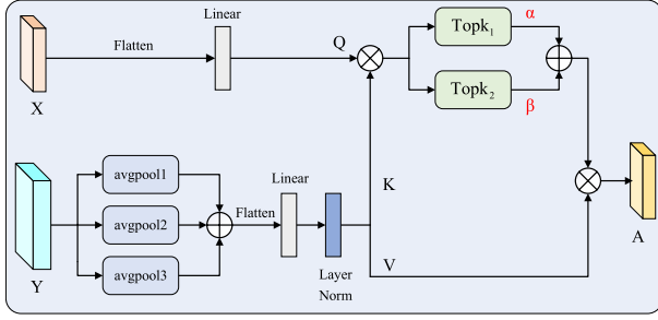
Fig. 4. Schematic of MSC. It first employs varying window sizes for average pooling to capture multiscale clues in the input data. Then, two TopK sparse operations are adopted to fuse the different features considering the irrelevant information.
