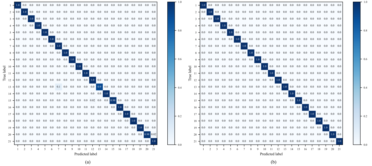
Fig. 14. Confusion matrices of MSCN counted on UCM dataset. The scene categories corresponding to the numbers are consistent with Fig. 7. (a) Confusion matrix for 50% training. (b) Confusion matrix for 80% training.
