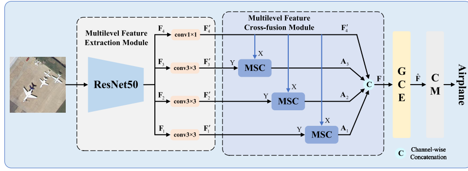
Fig. 3. Framework of MSCN. It consists of four parts: an MFEM, an MFCM, a GCE, and a CM.
