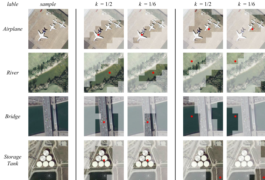
Fig. 12. Visualization results of TopK in MSC. The red dot area in the figure represents the query information, the semitransparent masked regions indicate the discarded information, and the remaining information is retained for feature fusion.
