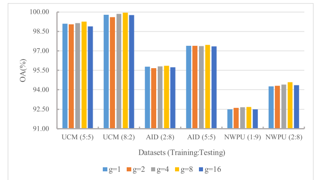
Fig. 13. OA values of different MSCNs with various g values counted on the UCM, AID, and NWPU datasets.
