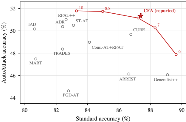
CIFAR-10
