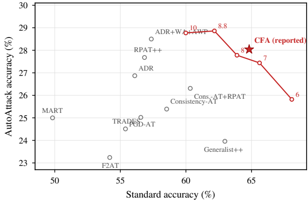
CIFAR-100
