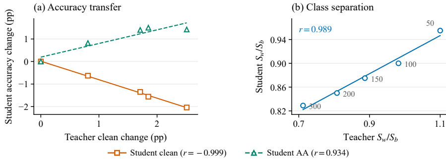
Figure 3: Transfer from clean self-teachers at different stages of training on CIFAR-100 (ResNet-18). (a) Changes in teacher clean accuracy and resulting student clean accuracy and AA relative to the 50-epoch teacher. (b) Ratio of within-class scatter S_w to between-class scatter S_b for teacher and student features. S_w measures the dispersion of features around their corresponding class centroids, whereas S_b measures the separation among class centroids; lower S_w/S_b indicates more compact within-class features relative to between-class separation. Labels denote teacher epochs, and lines are least-squares fits. Exact values are reported in Table 9.
