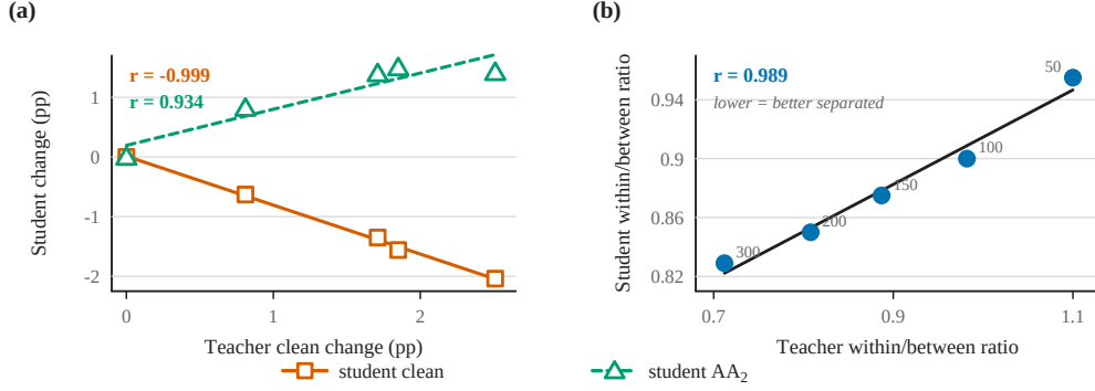
Figure 3: Accuracy and representation geometry across natural-teacher checkpoints on CIFAR-100 with ResNet-18. (a) Changes in student clean and AA 2 accuracy against the change in teacher clean accuracy, with all values measured relative to the 50-epoch checkpoint. (b) Student versus teacher within-to-between scatter ratio across the same five checkpoints; smaller values indicate stronger class separation. Lines are least-squares fits and r denotes the Pearson correlation. Exact values are reported in Table 10.
