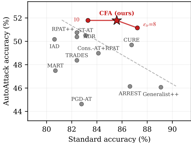
CIFAR-10
