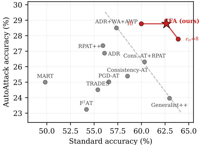
CIFAR-100
