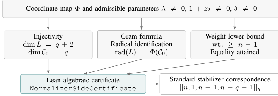
Figure 6: Dependencies of the algebraic certificate.
