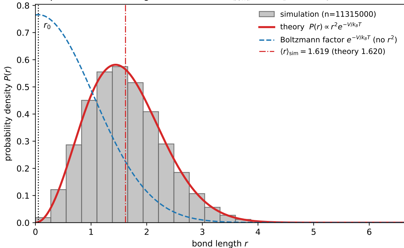
Equilibrium bond-length distribution ( k_{\text{bond}} = 1 , k_B T = 1 , r_0 = 0.0524492 )
