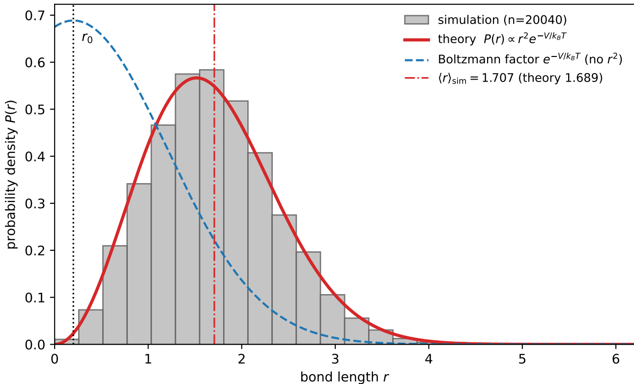
Equilibrium bond-length distribution ( k_{\text{bond}} = 1 , k_B T = 1 , r_0 = 0.2 )
