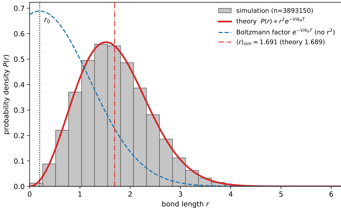
Equilibrium bond-length distribution ( k_{\text{bond}} = 1 , k_B T = 1 , r_0 = 0.2 )
