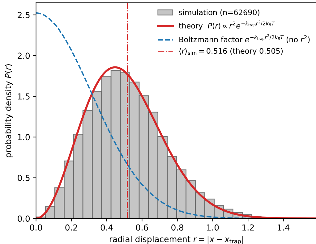
Radial displacement ( k_{\text{trap}} = 10, k_B T = 1 )
