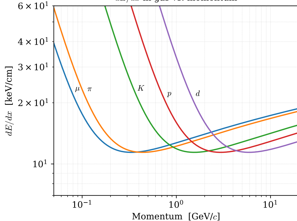
dE/dx in gas vs. momentum
