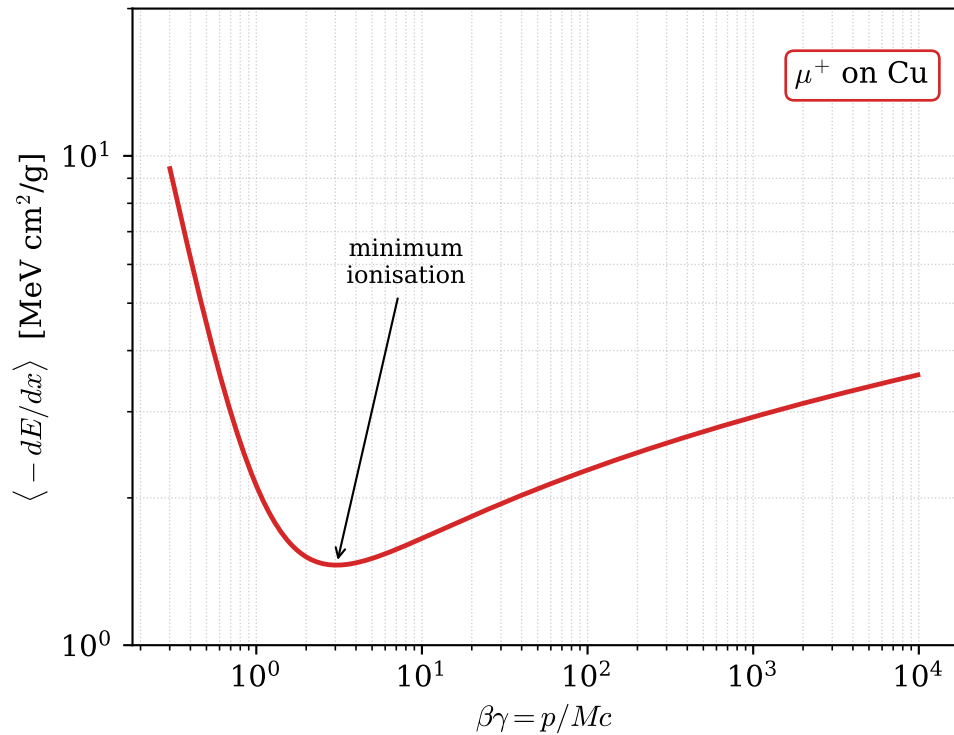
Mass stopping power (Bethe region)
