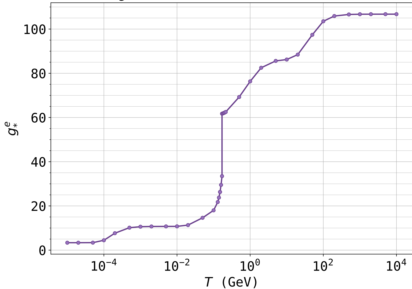
g_*^e , QCD transition at 170 MeV
