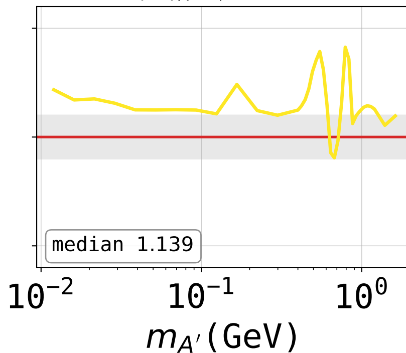
5: \langle\sigma v\rangle_f , x_f from \Gamma=H
