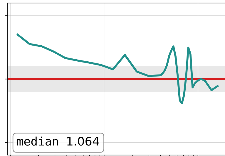
3: relic \sigma_0 , x_f=20
