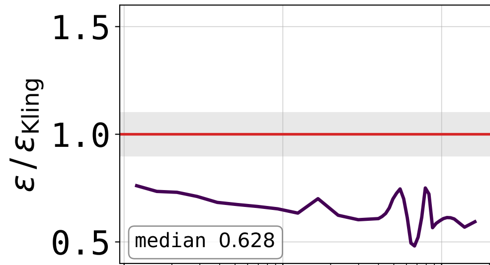
1: fixed \langle\sigma v\rangle , x_f=20
