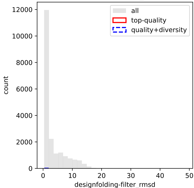
designfolding-filter_rmsd
