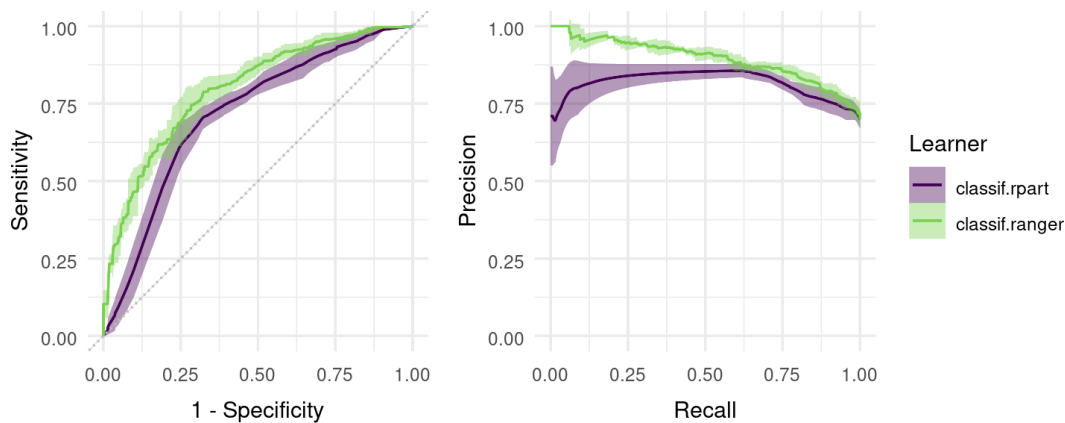
Figure 3.16: Comparing random forest (green) and decision tree (purple) using ROC and PR Curves.
