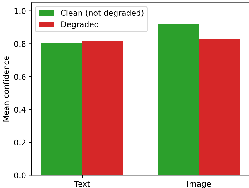
Public CrisisMMD domain: confidence gap is weak (image) or reversed (text) on real data
