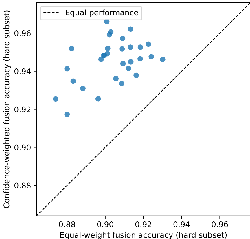
Confidence-weighted fusion wins in 30/30 independent splits
