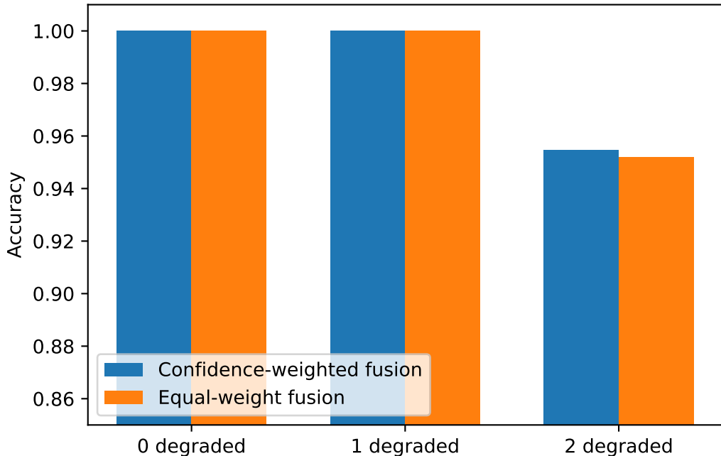
IT-incident domain: fusion strategies by degradation count
