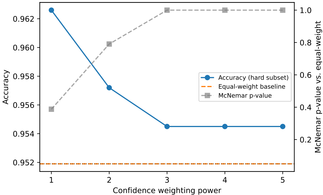
IT-incident domain: weighting sharpness sweep
