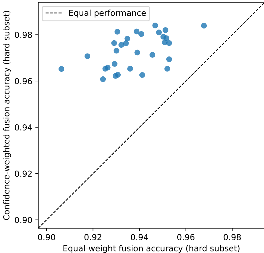
IT-incident domain: CW wins in 30/30 independent splits
