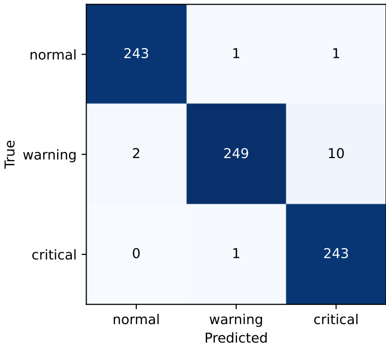
Confidence-weighted fusion (test split)
