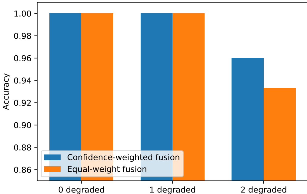
Fusion strategies only differ when 2 modalities are degraded
