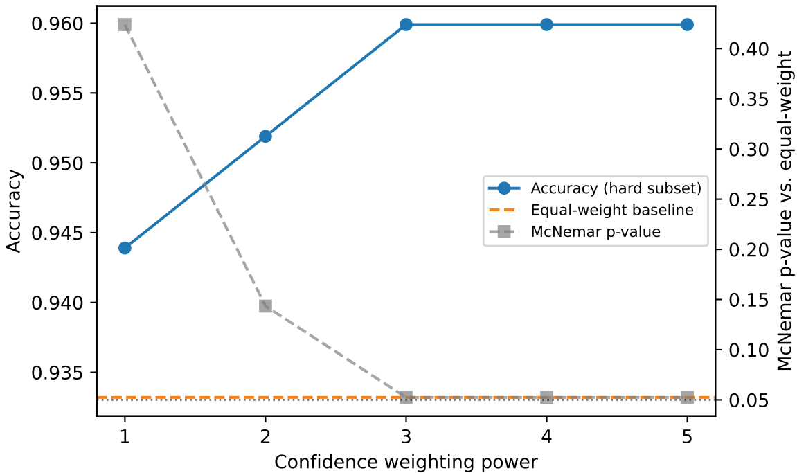
Weighting sharpness sweep: plateaus at power=3
