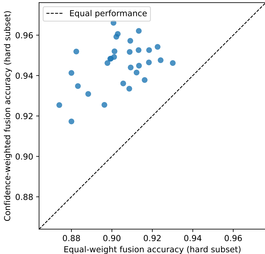
Confidence-weighted fusion wins in 30/30 overlapping partitions
