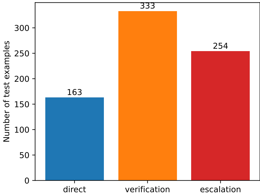
Dynamic planner: strategy selection distribution
