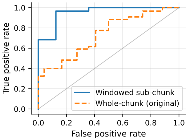
Stage 2 indirect-injection detection ROC
