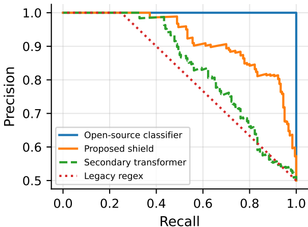
Stage 1 injection detection PR curve
