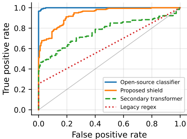
Stage 1 injection detection ROC
