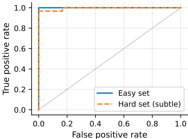
Stage 3 hallucination ROC: easy vs. hard set
