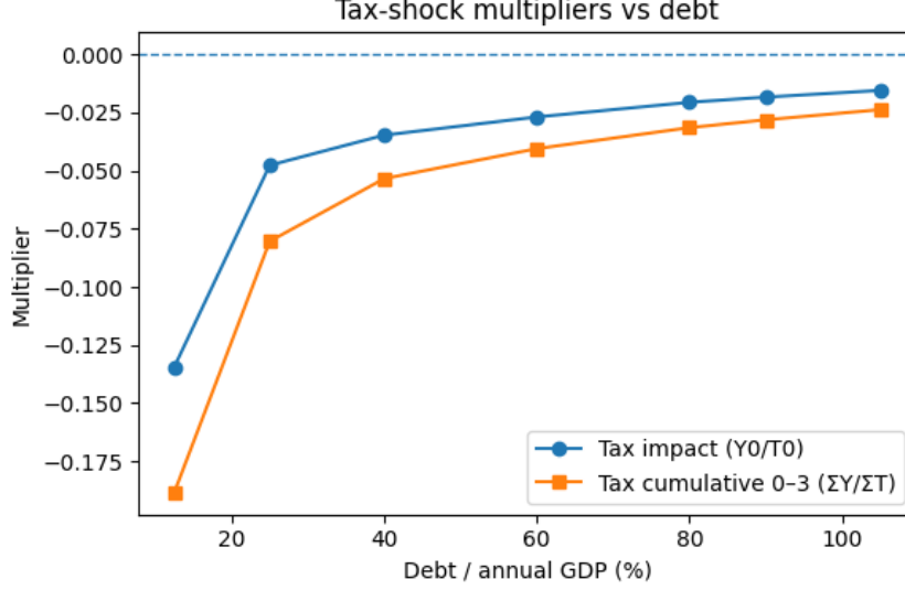
Figure 32: Impact and short-run cumulative tax multipliers as a function of the debt-to-annual-GDP ratio.
