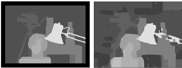
Figure 2. Ground truth Tsukuba stereo set disparity map (left) and Tsukuba stereo set disparity map generated with initial CUDA implementation (right).
