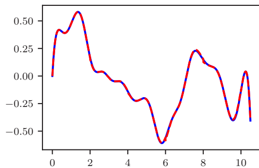
Trajectory Reconstruction
