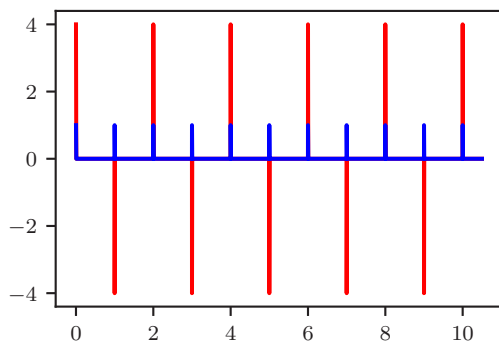
Kernel Inversion
