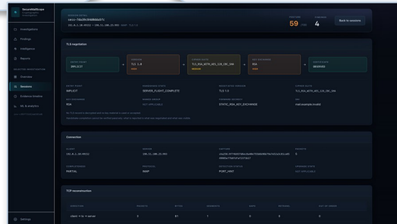
Session negotiation
