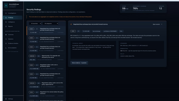
Findings triage
