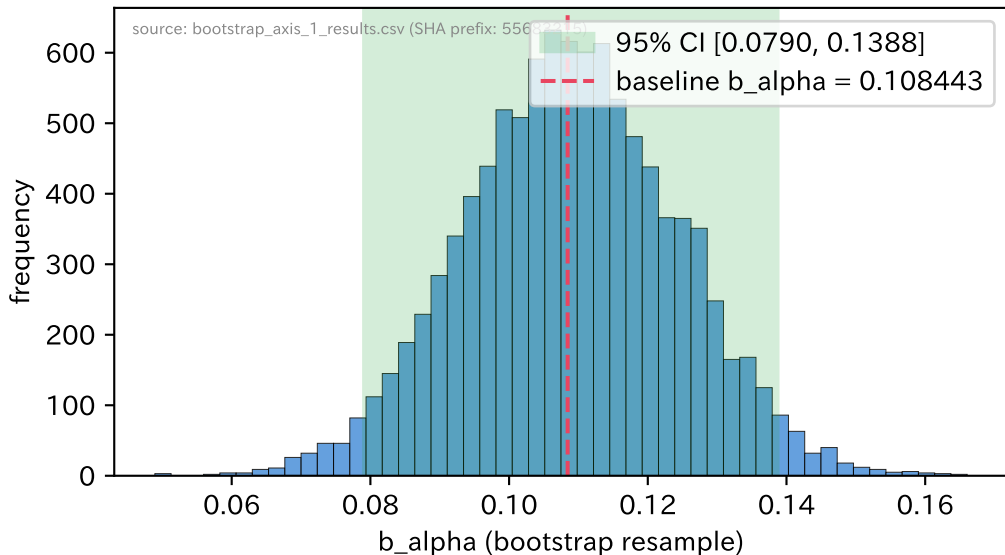
axis_1 SPARC b_alpha bootstrap distribution (N=10,000 resamples, median=0.108781)
