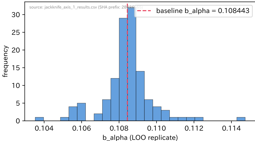
axis_1 SPARC b_alpha jackknife LOO distribution (N=124, 3sigma outliers=0, std_loo=0.001389)
