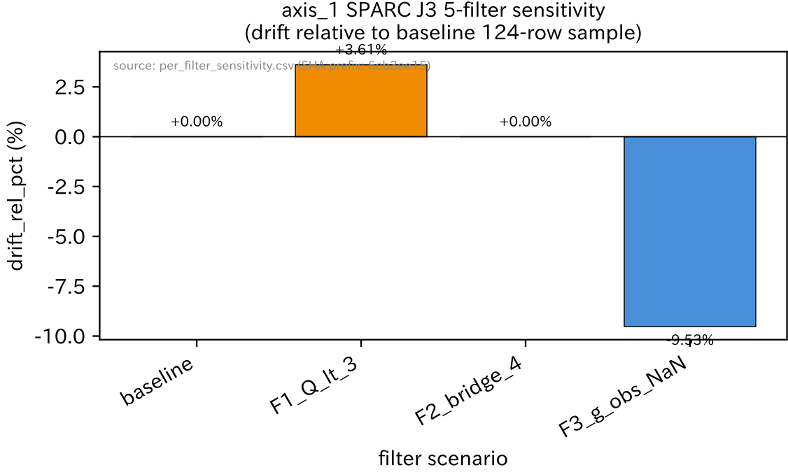
図 3 axis_1 SPARC J3 5-filter sensitivity. drift_rel_pct (%) per filter scenario relative to canonical 124-row baseline. Filter 1 ( Q < 3 disable, n_{\text{after}} = 129 ) shows +3.61% drift, providing direct forensic evidence that the Phase 1a Q -column patch is the causal mechanism for the v1.0.3.1 deviation fix. Other filter toggles confirm independence of canonical structural cuts from the central b_{\alpha} estimate. Source: per_filter_sensitivity.csv (SHA-256 prefix: 6cb3ee15...).
