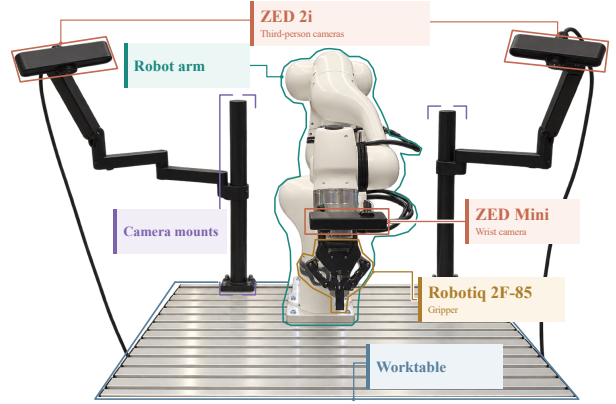
Figure 4. Real-robot evaluation setup. A Franka Research 3 with a Robotiq 2F-85 gripper operates over the worktable. A ZED Mini provides the wrist view, while two ZED 2i cameras provide third-person views. The same robot and camera arrangement is used in both evaluation protocols.
