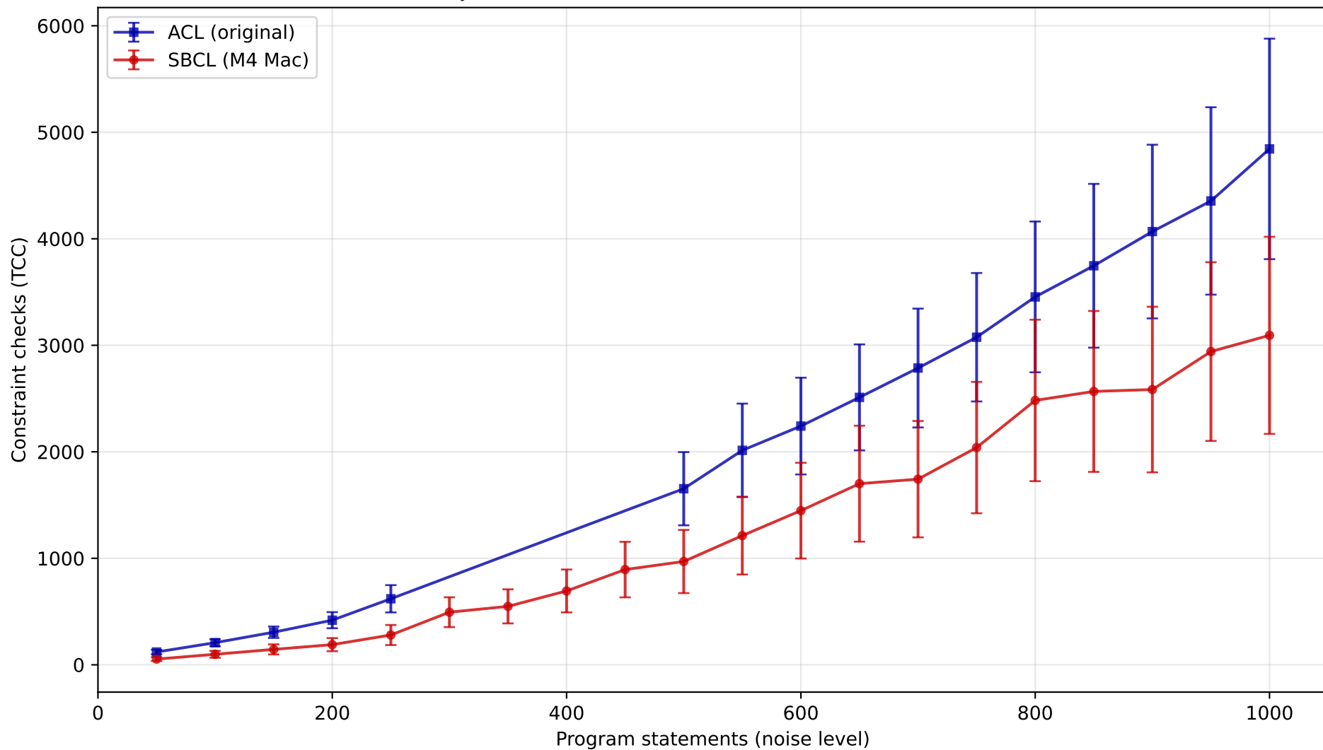
ij4: MAP-CSP FCDR w/ adv sort -- ACL vs SBCL
