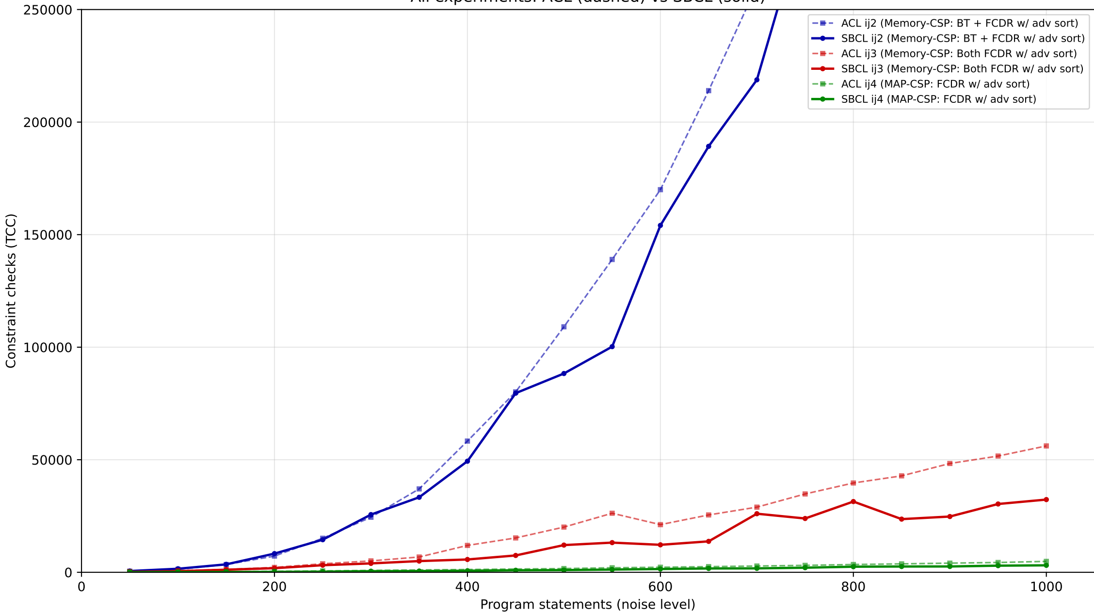
All experiments: ACL (dashed) vs SBCL (solid)
