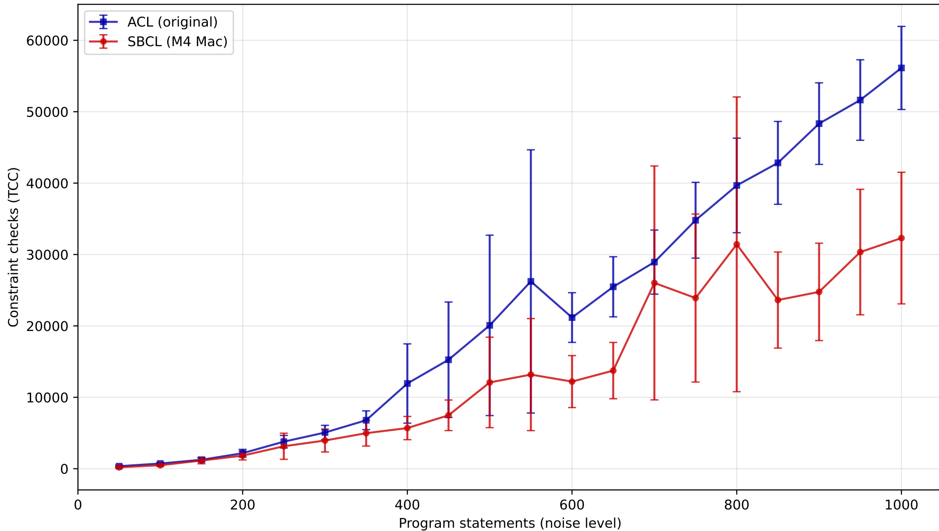
ij3: Memory-CSP Both FCDR w/ adv sort -- ACL vs SBCL
