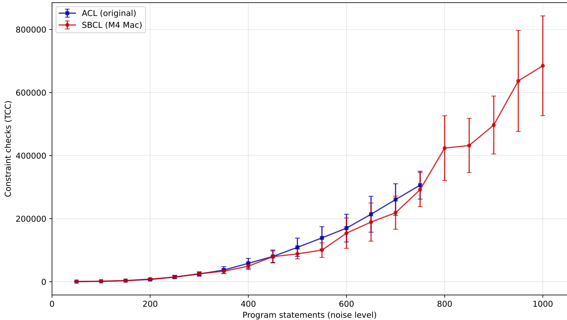
ij2: Memory-CSP BT + FCDR w/ adv sort -- ACL vs SBCL
