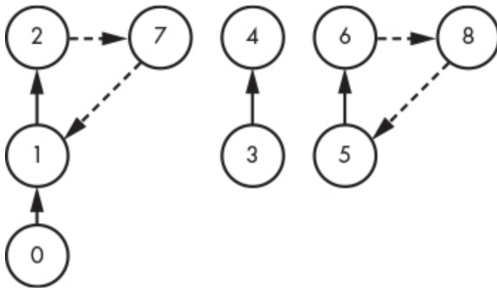
Figure 8-9: The data structure after another SetEnemies operation
