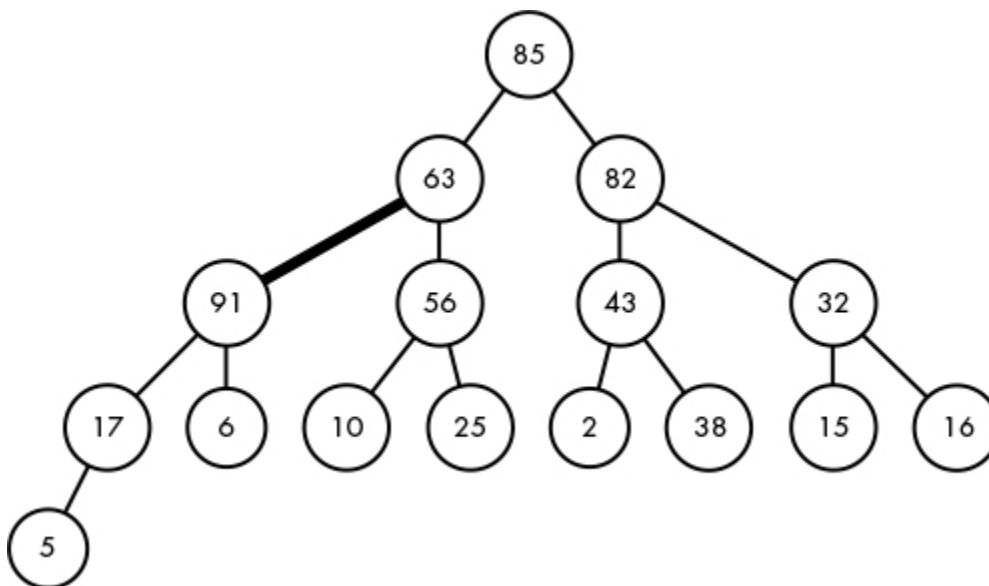
Figure 7-7: A max-heap with 91 moved up again
