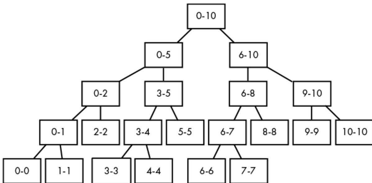
Figure 7-17: A segment tree for an 11-element array
