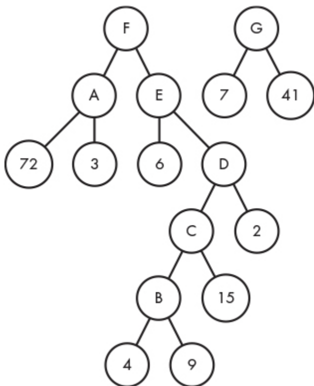
Figure 2-3: A tree split in two
