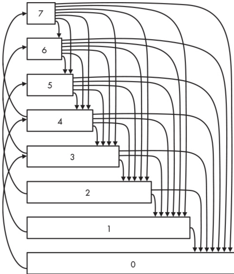
Figure 4-5: Graph of Bob's moves
