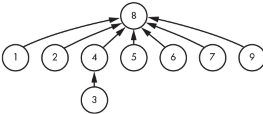
Figure 8-6: An example of path compression
