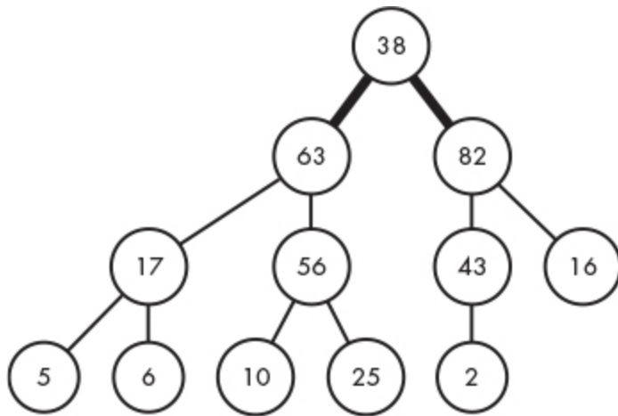
Figure 7-10: A max-heap with 85 extracted
