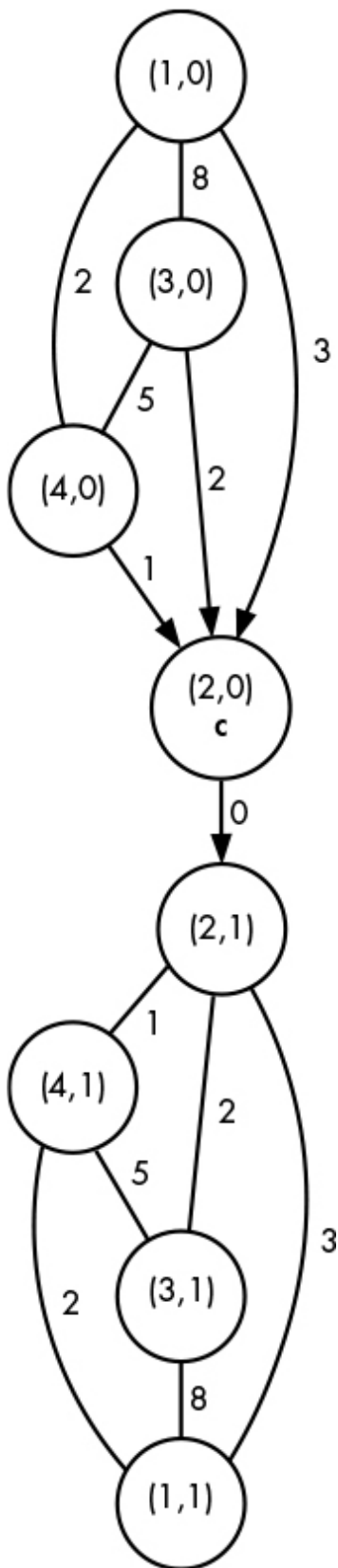
Figure 5-5: A grandma graph with a cookie state
