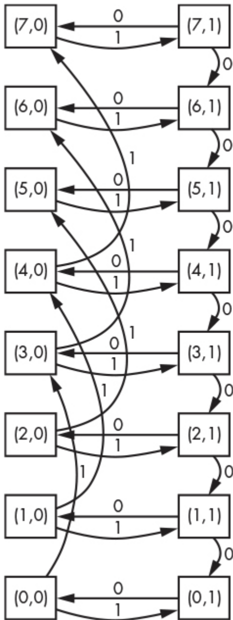
Figure 4-6: Graph of Bob's moves using two ropes
