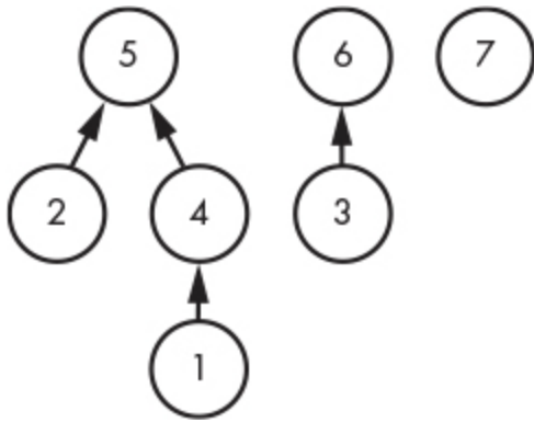
Figure 8-1: A tree-based union-find data structure
