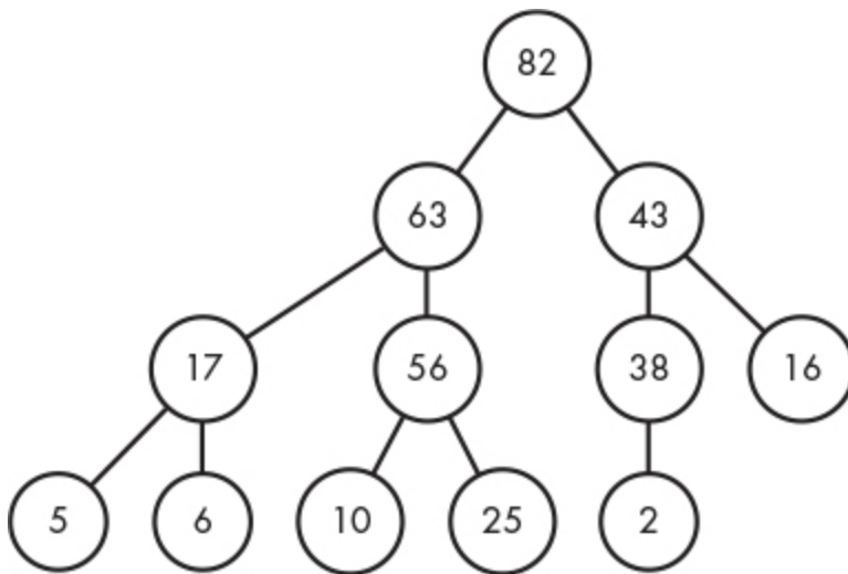
Figure 7-12: A max-heap with 38 moved further down
