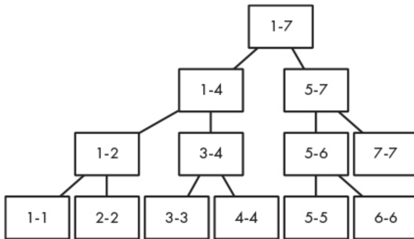
Figure 7-19: A segment tree for a seven-element array
