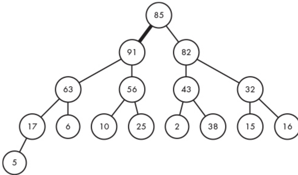
Figure 7-8: A max-heap with 91 moved up yet again
