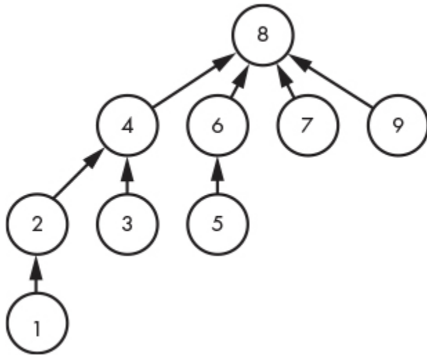
Figure 8-5: A bad case of union by size
