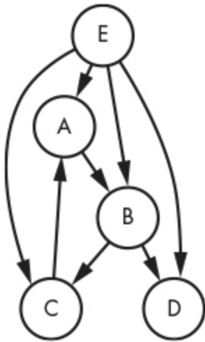
Figure 4-2: A directed graph
