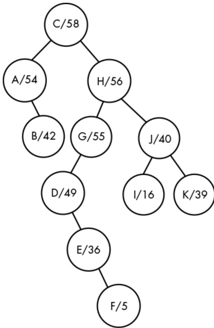
Figure 7-15: A treap
