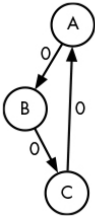
Figure 5-6: A graph with an infinite number of shortest paths
