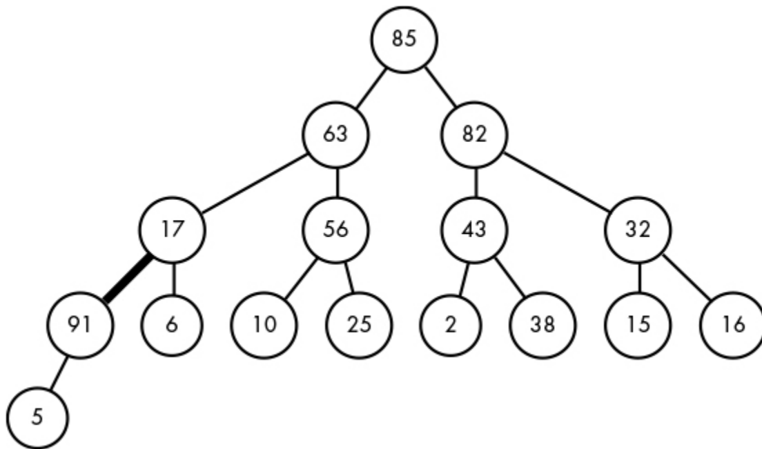
Figure 7-6: A max-heap with 91 moved up
