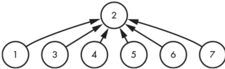
Figure 8-4: An optimized tree-based union-find data structure
