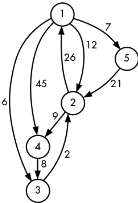
Figure 5-1: The Mice Maze graph
