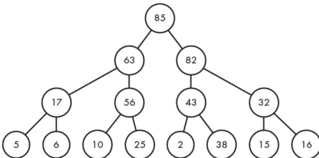
Figure 7-4: A max-heap with the max-heap-order violation repaired
