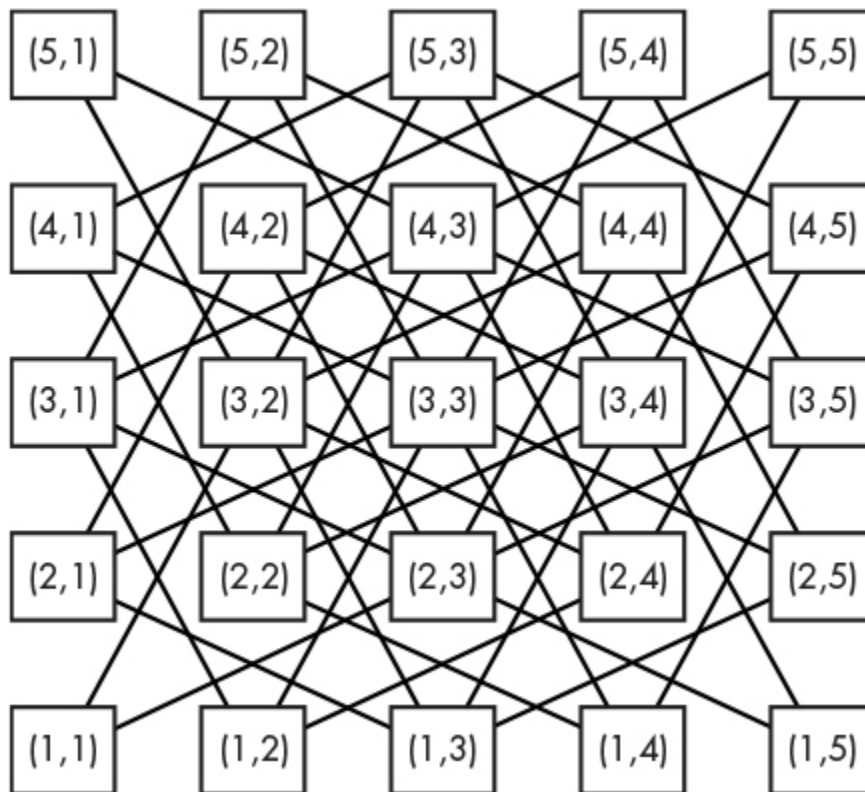
Figure 4-1: Graph of knight moves
