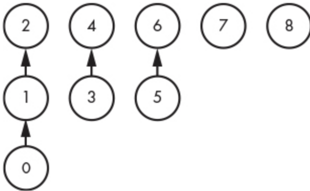
Figure 8-7: The data structure after four SetFriends operations
