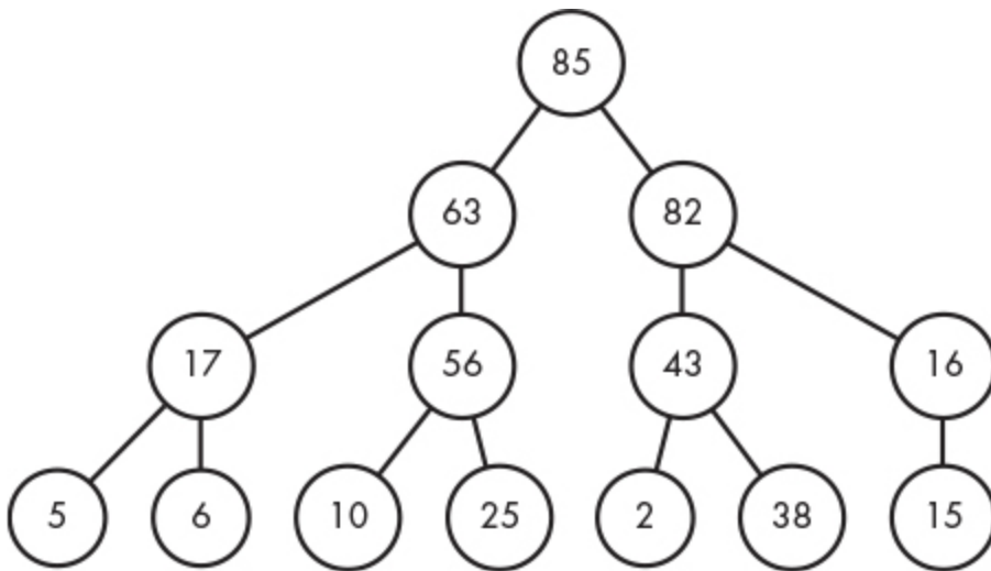
Figure 7-2: A max-heap with 15 inserted
