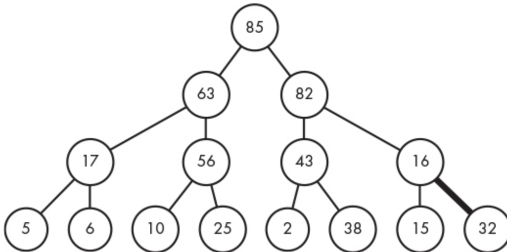
Figure 7-3: A max-heap with 32 inserted
