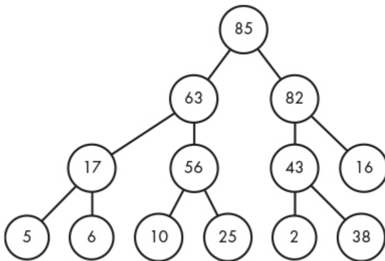
Figure 7-1: A max-heap
