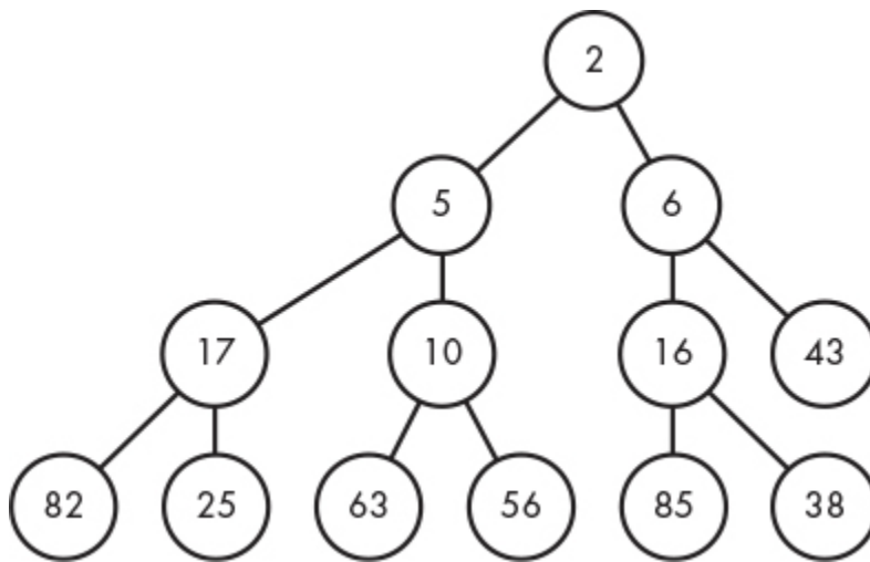
Figure 7-14: A min-heap
