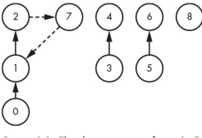
Figure 8-8: The data structure after a SetEnemies operation
