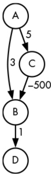
Figure 5-3: A graph with a negative-weight edge
