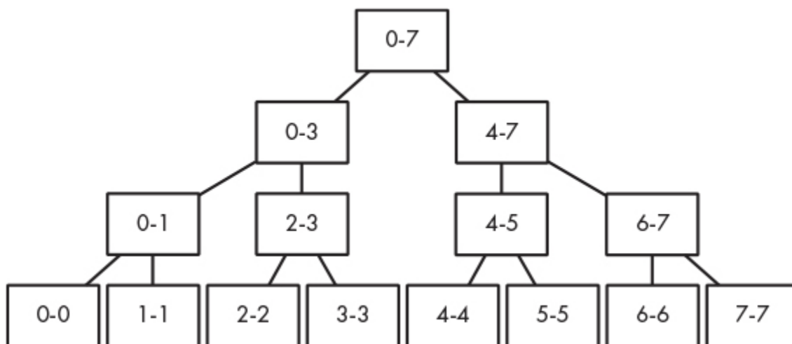
Figure 7-16: A segment tree for an eight-element array
