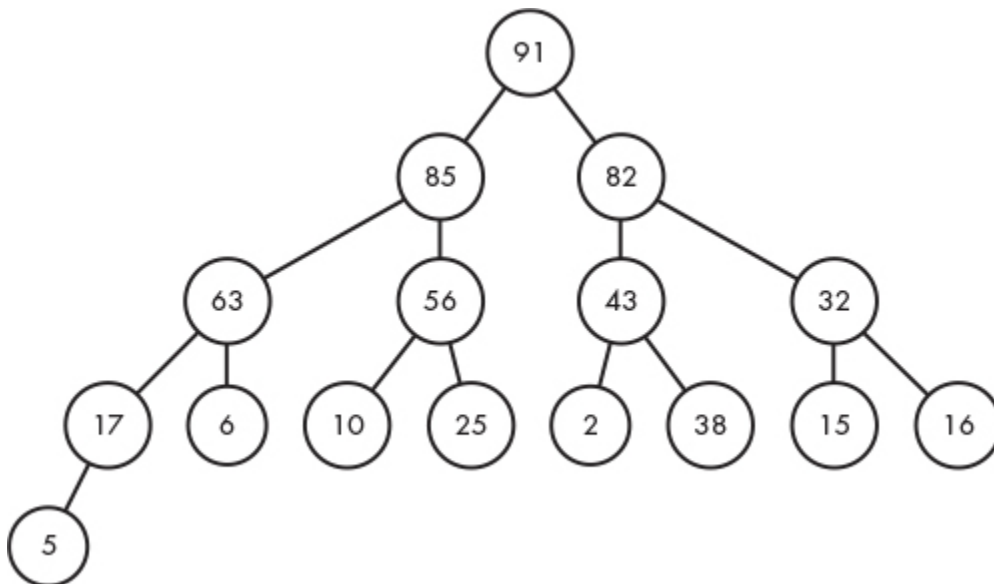
Figure 7-9: A max-heap with the heap-order violation repaired
