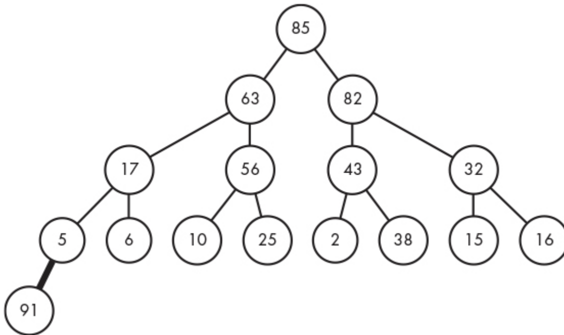
Figure 7-5: A max-heap with 91 inserted
