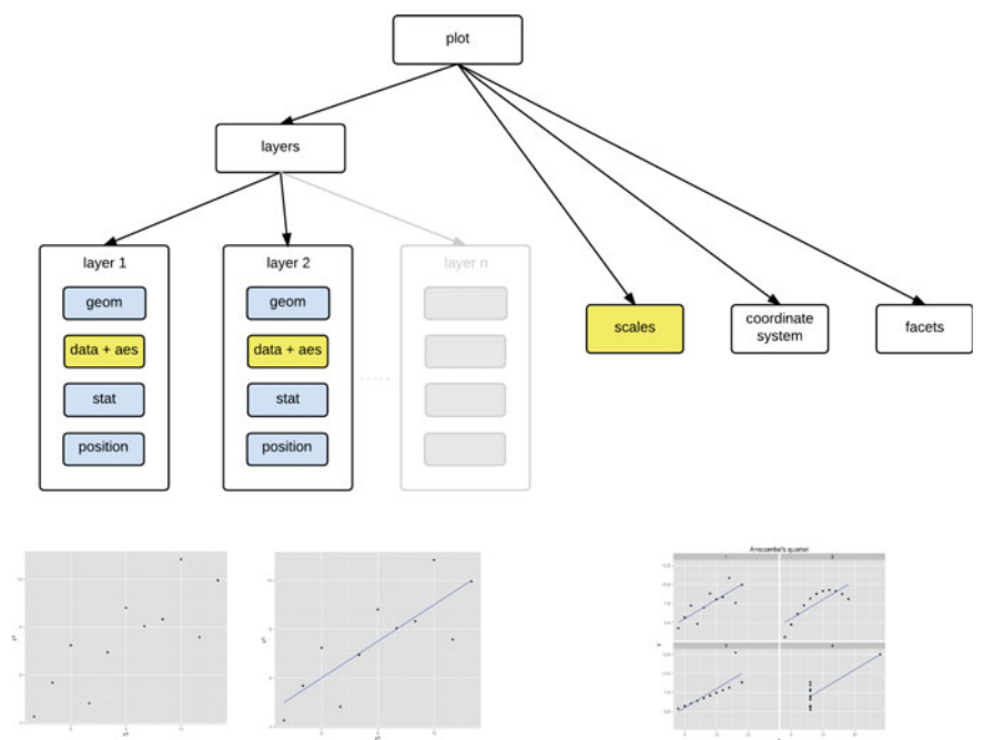
Fig. 3.3 A schematic illustrating the structure of plots. A layer is defined by an R data frame and its aesthetic properties, a geometric object to visually represent that summary, and an optional position adjustment to move overlapping geometric objects out of their way and a statistical approach to summarize the rows of that data frame. Scales affect the data+aes defined in the layers of a plot
