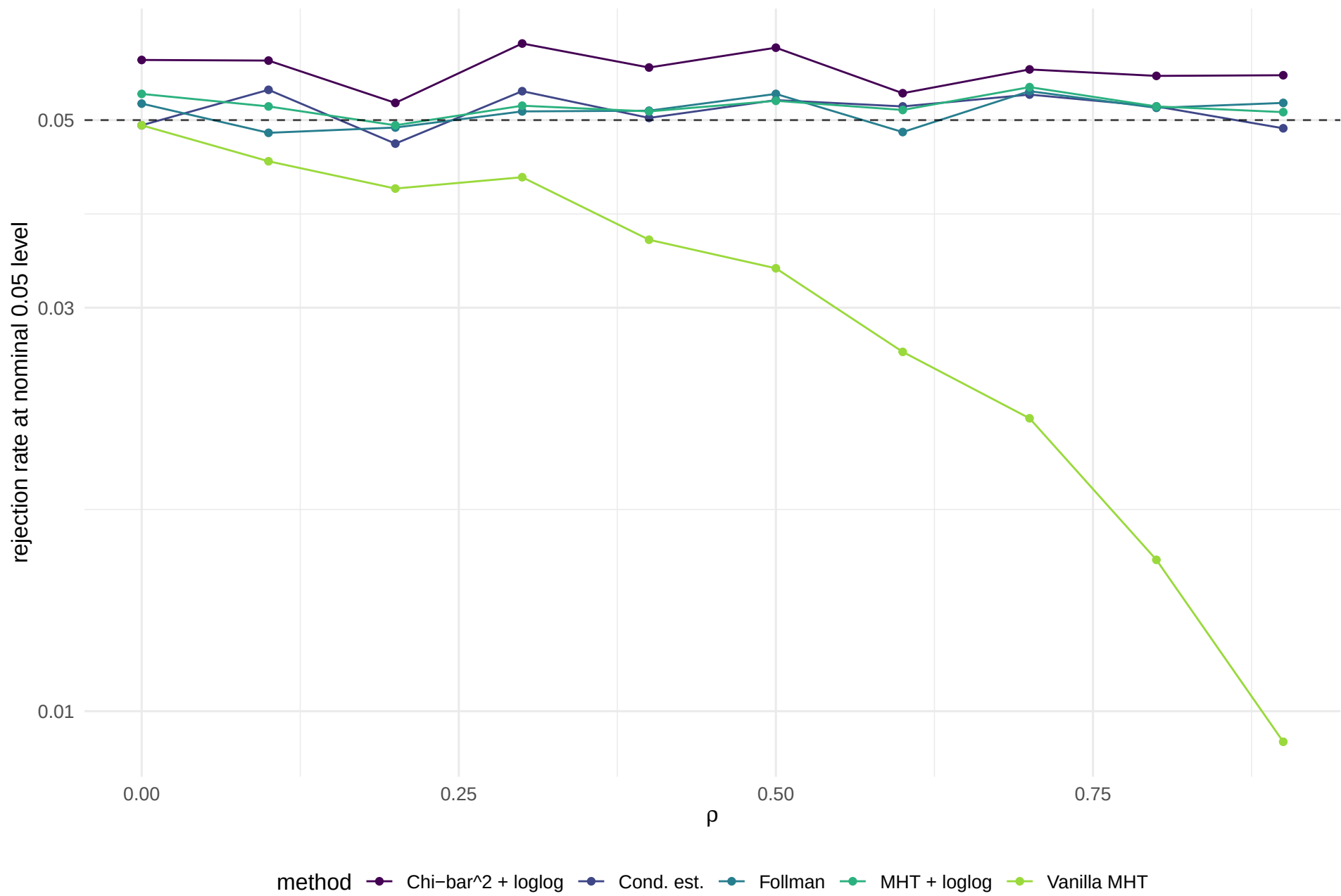
rejection rate of tests under the null
