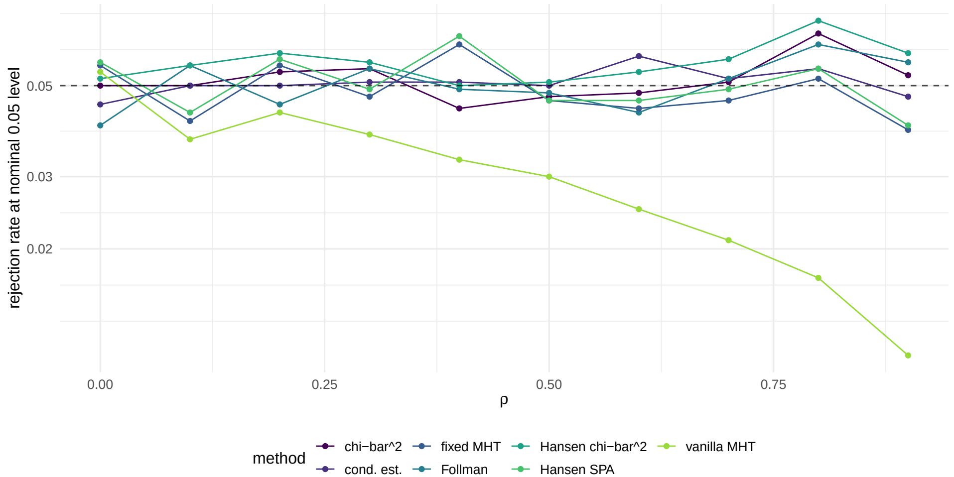
rejection rate of tests under the null
